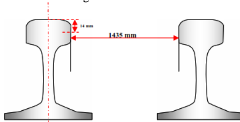
Figure 11. Railway width 1435 mm
