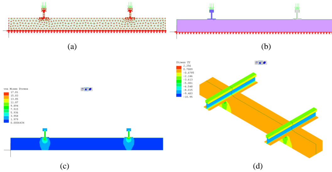
Figure 13. Stress Behaviour of Concrete Bearing
