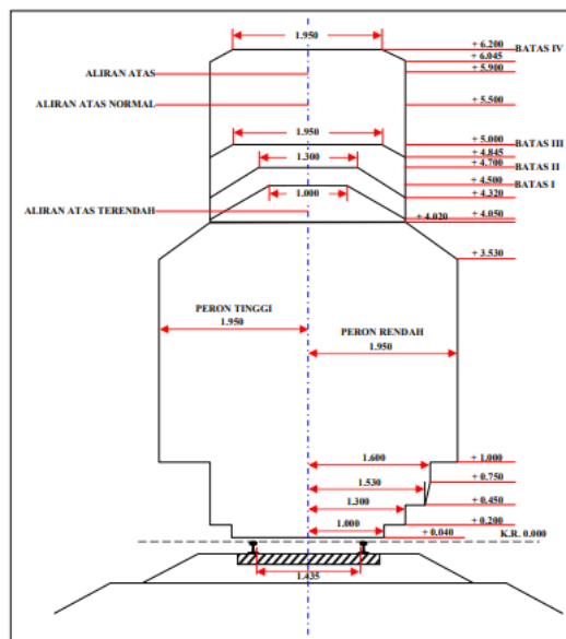
Figure 1. The position of laying the railroad tracks on the bearings
