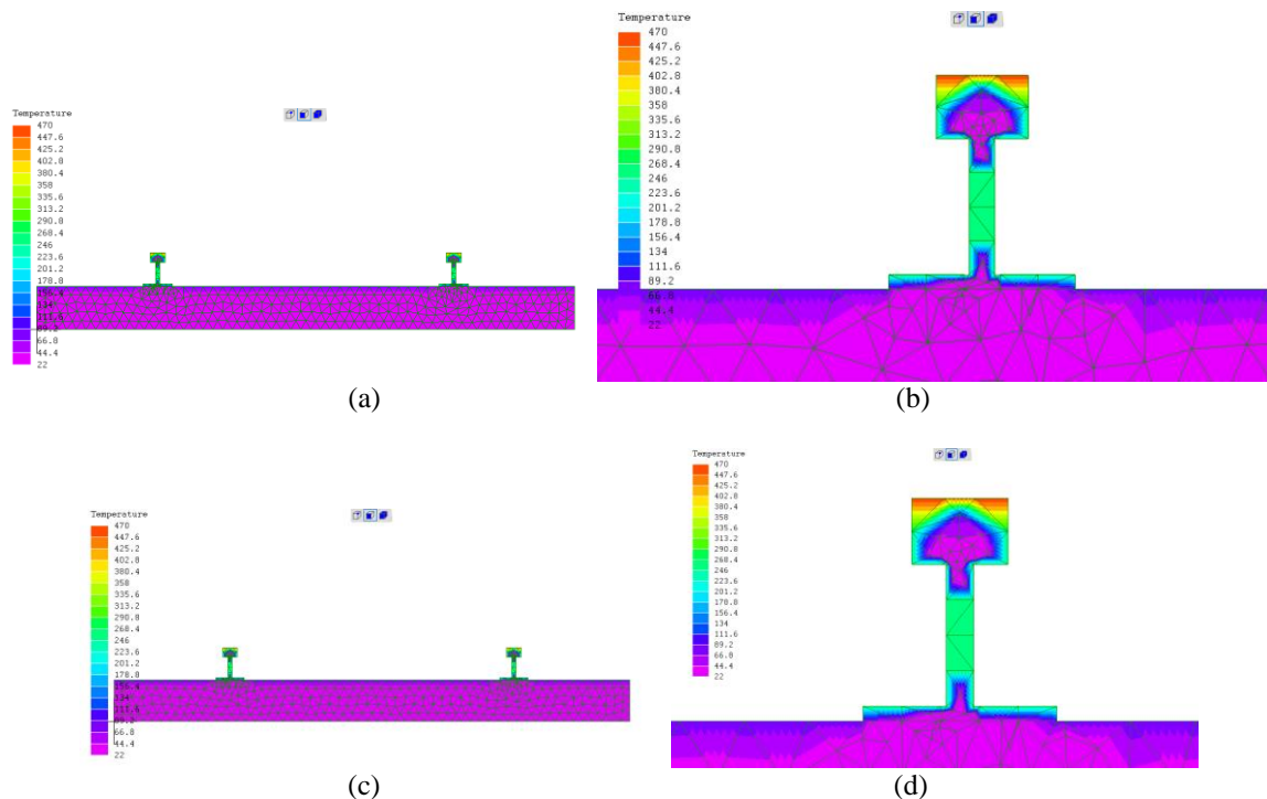
Figure 16. Temperature behaviour of bearing (a)(b) Concrete Bearing (c)(d) Wood Bearing
