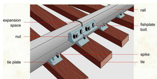
Figure 4. Railroad track components (source: www.infovisual.info )
