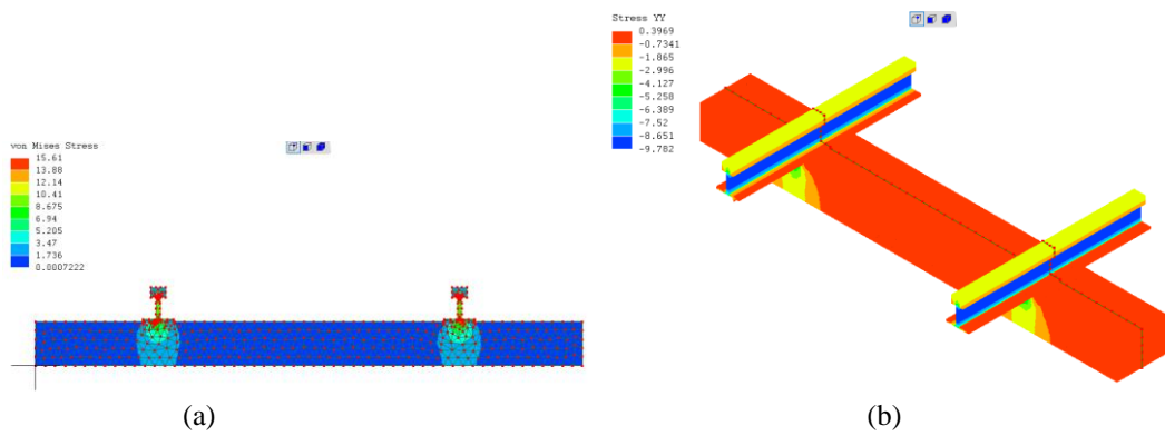
Figure 14. Stress Behaviour of Wood Bearing
