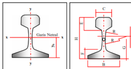
Figure 3. Rail dimensions
